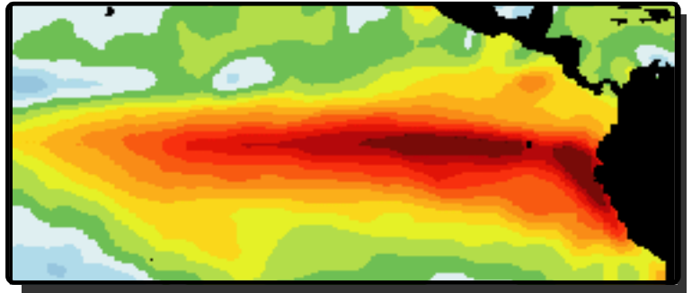
El Niño is the abnormal warming of ocean temperatures in the eastern tropical Pacific Ocean. La Niña is the opposite - the cooling of ocean temperatures in the tropical Pacific. These patterns, which occur every 2- 7 years, affect the climate in North Carolina.
