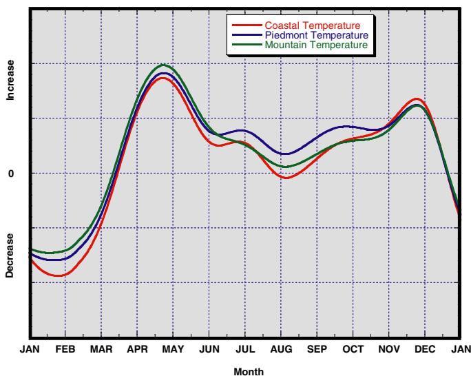
Change in Temperature during El Niño Events
