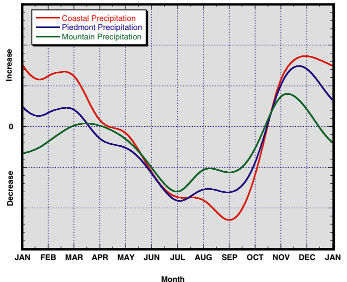
Change in Precipitation During El Niño Events
